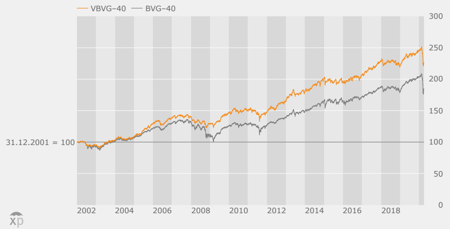
Fundo VBVG-40 vs BVG-40 01.01.02–31.03.20
