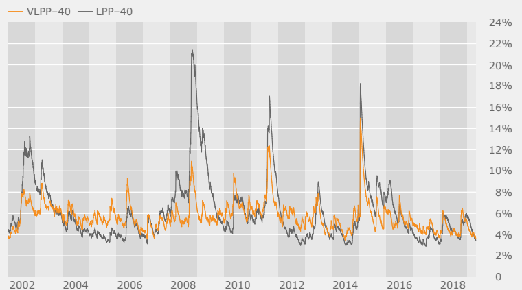
VLPP-40 vs LPP-40 Ex Post Volatility 01.01.02–30.04.19
