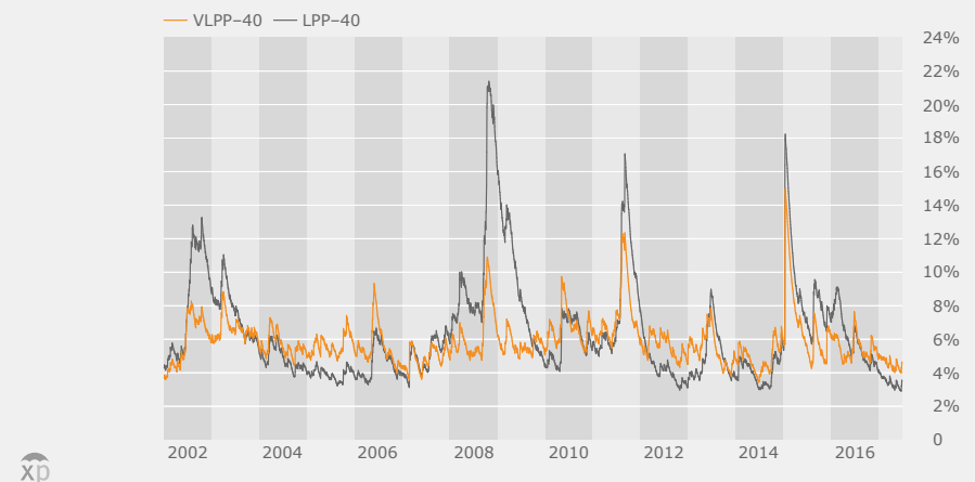
VLPP-40 vs LPP-40 Ex Post Volatility 01.01.02–30.06.17
