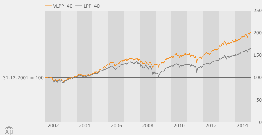
Fundo VLPP-40 vs LPP-40 01.01.02–31.12.14
