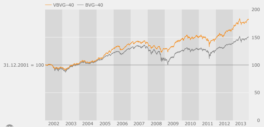
Fundo VBVG-40 vs BVG-40 01.01.02–29.11.13
