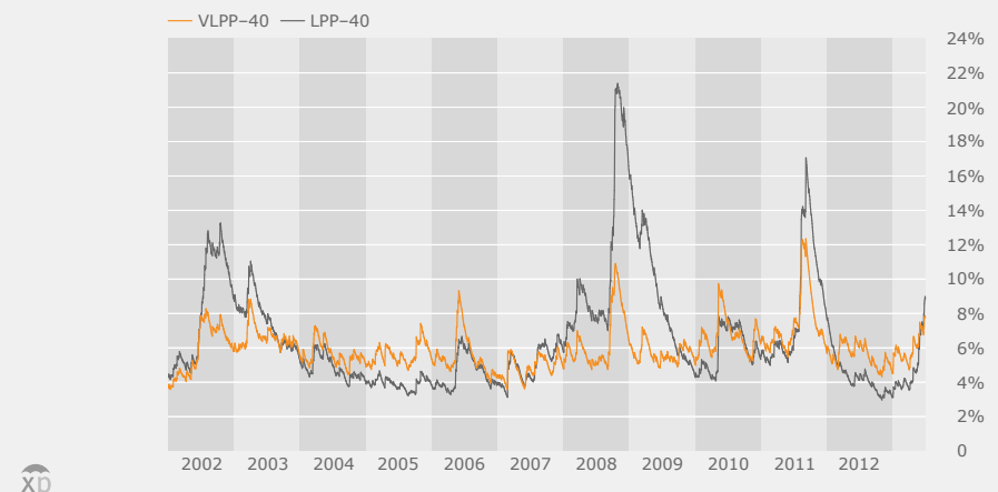
VLPP-40 vs LPP-40 Ex Post Volatility 01.01.02–28.06.13
